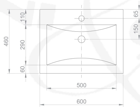
Top View - Basin
