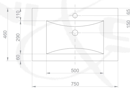
Top View - Basin
