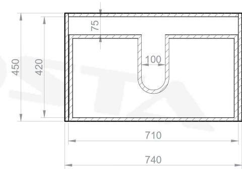
Horizontal Section - Cabinet
