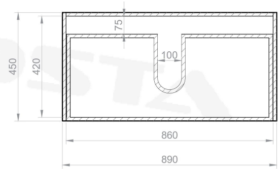
Horizontal Section - Cabinet
