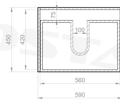
Horizontal Section - Cabinet
