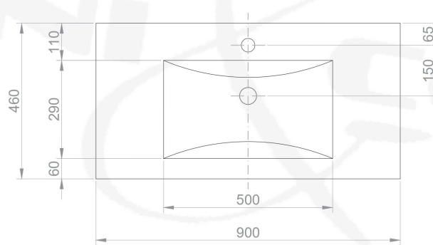
Top View - Basin
