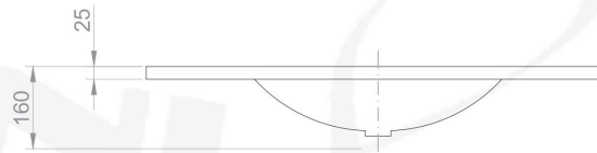
Front View - Basin
